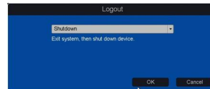
Figure 2-10 Shutdown
