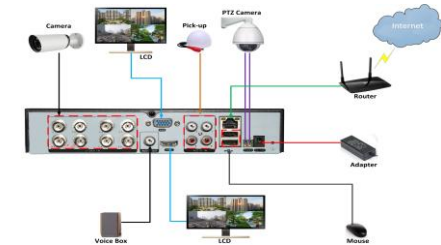
Figure 2-1 Device Connection
