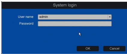
Figure 2-2 Login
