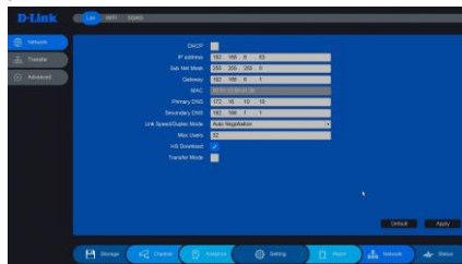
Figure 2-7 Network setting
