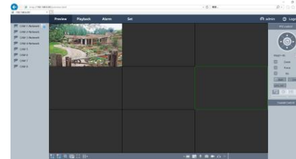
Figure 2-8 WEB
