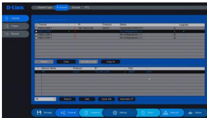
Figure 2-4 Add cameras
